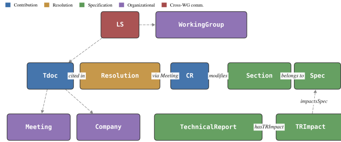
Fig. 2. SPECTRA core schema (reader-facing labels). Central row: traceability spine \text{Tdoc} \rightarrow \text{Resolution} \rightarrow \text{CR} \rightarrow \text{Section} \rightarrow \text{Spec} . Formal OPs are references (Resolution \rightarrow Tdoc, drawn reversed), modifiesSection (CR \rightarrow Section), and belongsToSpec (Section \rightarrow Spec). The Resolution \rightarrow CR step is drawn lightly because no direct OP exists; the connection is reconstructed by joining shared Meeting , AgendaItem , and CRPack context. Dashed grey arrows carry secondary OPs (LS \rightarrow WG via sentTo ; Tdoc \rightarrow {Meeting, Company}) and one class-hierarchy edge (LS \sqsubseteq Tdoc). The TR \rightarrow TRImpact \rightarrow Spec reified chain is shown explicitly. Section hierarchy edges ( hasSubSection/parentSection , irreflexive + asymmetric) and the four intra-section / TR cross-reference irreflexive OPs ( referencesSection/referencedBySection , referencesTR/referencedByTR ) are realized inside the Section/TR sub-trees.
