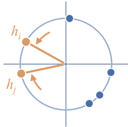
embeddings
