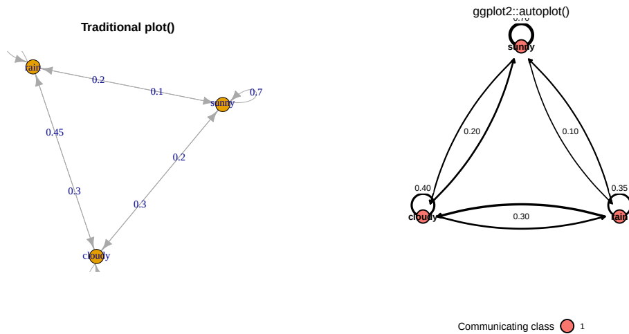
Figure 1: The same Markov chain represented with the traditional ‘plot’ method (left) and the optional ‘ggplot2’-based ‘autoplot’ method (right).
