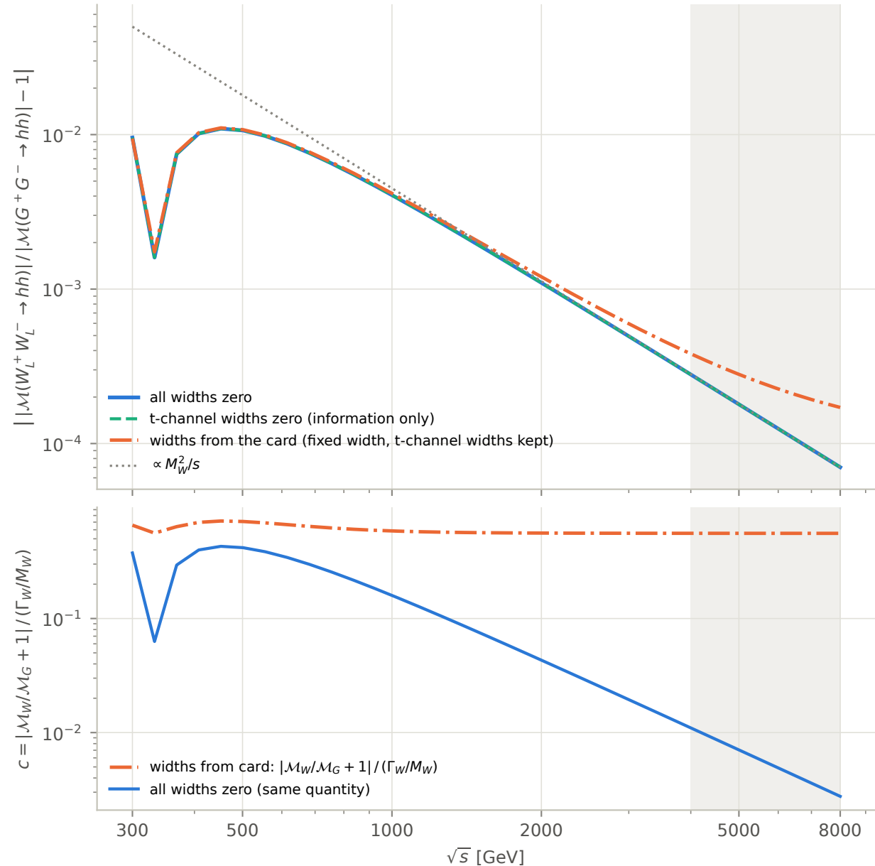
Goldstone equivalence, \theta = 90^\circ (MG5 sm, Feynman gauge); shaded: 4-8 TeV check window
