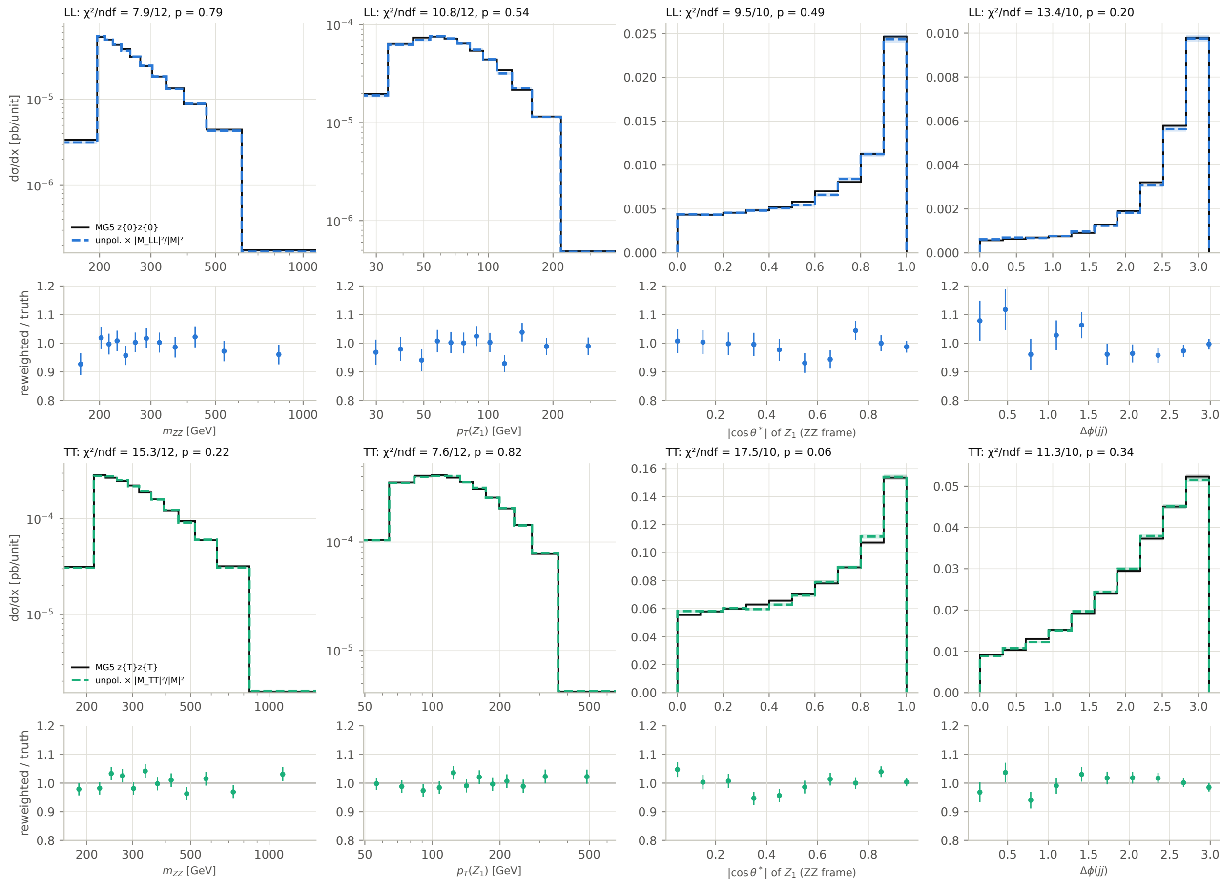
Closure of the external-Z polarisation reweighting (partonic CM) against MG5 polarised samples (m ZZ , p T : 12 equal-population bins; outer bins, reaching 0 and the maximum, drawn truncated)
