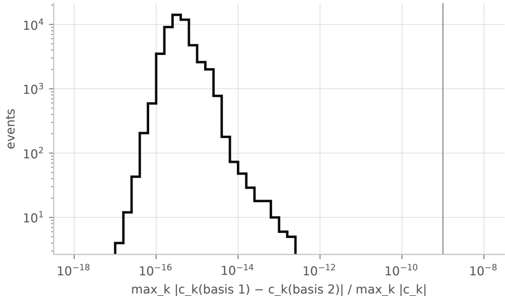
Coefficient stability, two independent bases
