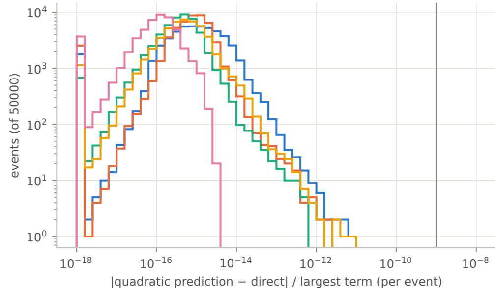
Morphing closure on all SM events
