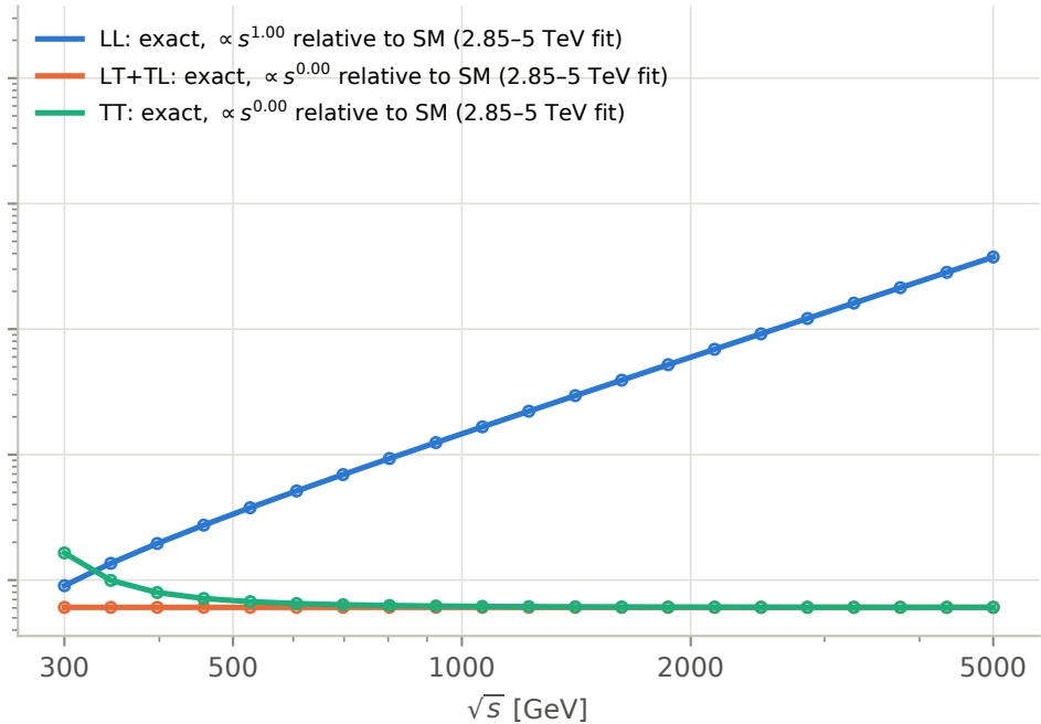
cHDD: SM \times EFT interference per W helicity class (lines exact, circles JAX)
