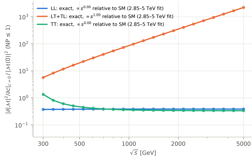
cHW: SM \times EFT interference per W helicity class (lines exact, circles JAX)
