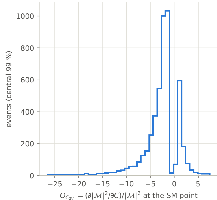
HHVBF pp \rightarrow hhjj SM sample (5000 events): matrix-element optimal observables from JAX gradients (checked to 5e-13)
