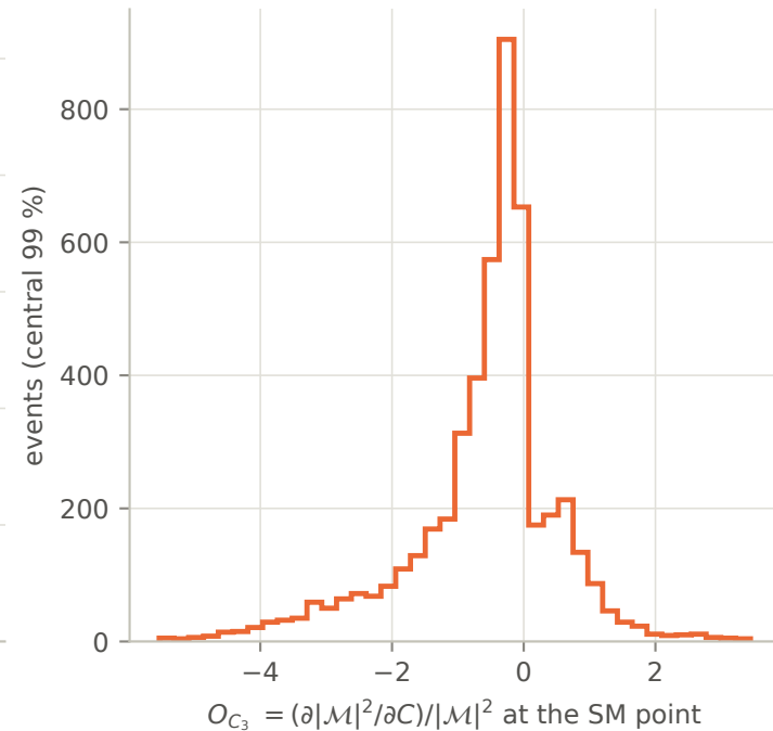
HHVBF pp \rightarrow hhjj SM sample (5000 events): matrix-element optimal observables from JAX gradients (checked to 5e-13)
