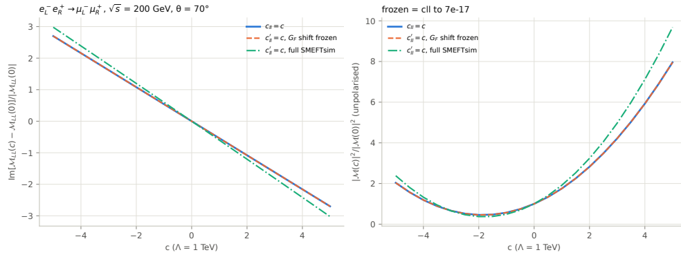
Figure 9: Study 5: the Fierz identity between the two four-lepton operators, and the effect of the input-scheme shift.
