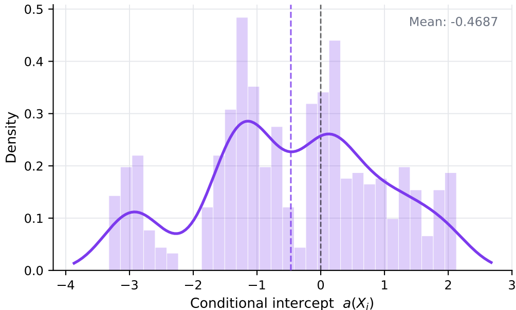
Distribution of Conditional Intercept a(X_i)
