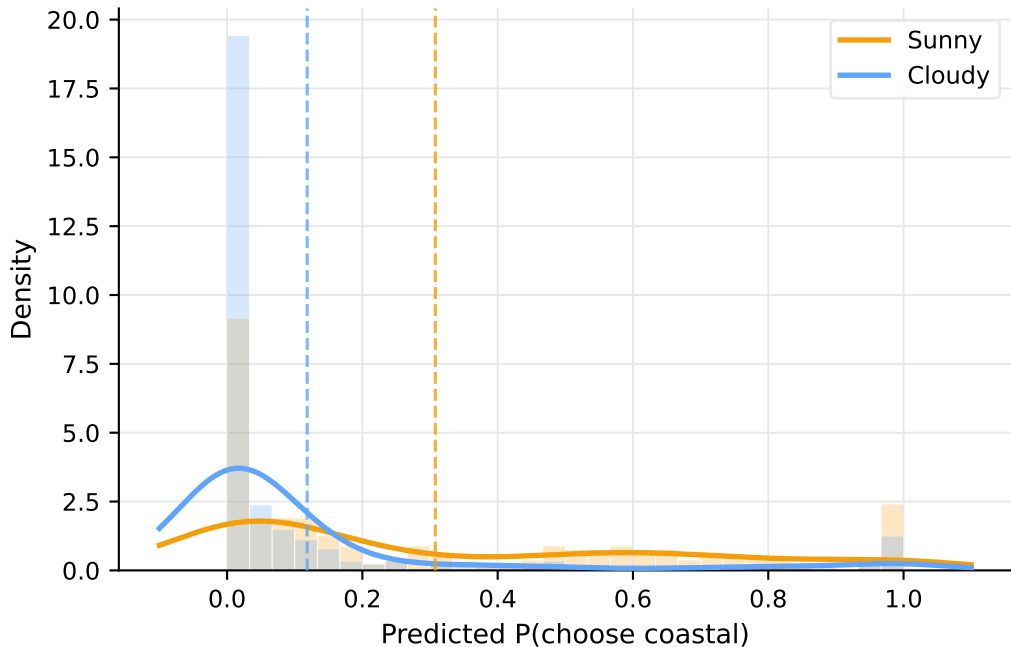
Predicted Coastal Probability by Weather Condition
