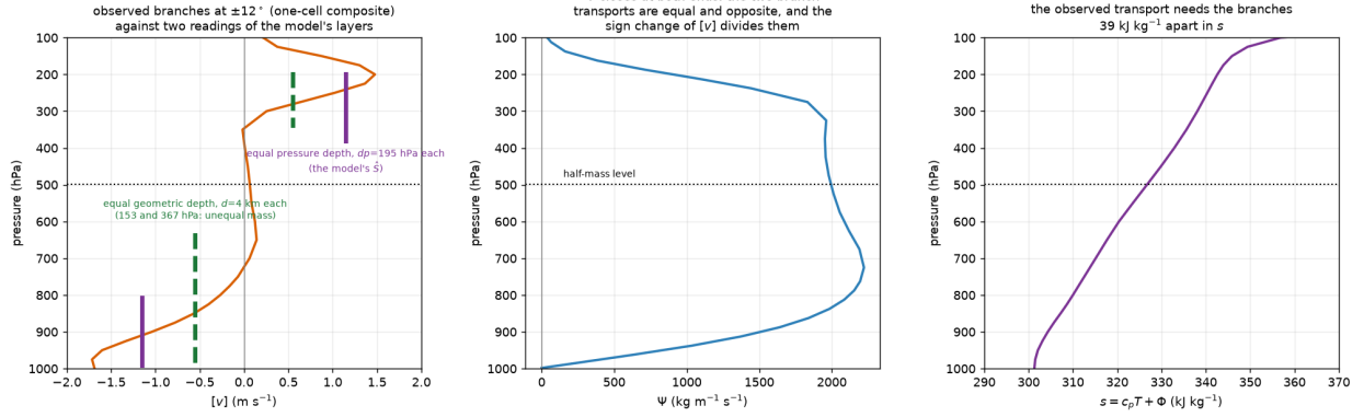
Figure 2: (a) The observed [v] at \pm 12^\circ , composited into one cell, with the model's two layers drawn two ways: equal geometric depth of 4 km each (green dashed, 153 and 367 hPa, unequal mass) and equal pressure depth of 195 hPa each (purple, the depth the model's \hat{S} implies). (b) \Psi vanishes at both ends once the column mass flux is removed, which is the statement that the two branch transports are equal and opposite; the level where [v] changes sign is what divides them. (c) The observed s(p) , whose branch contrast the transport must reproduce.
