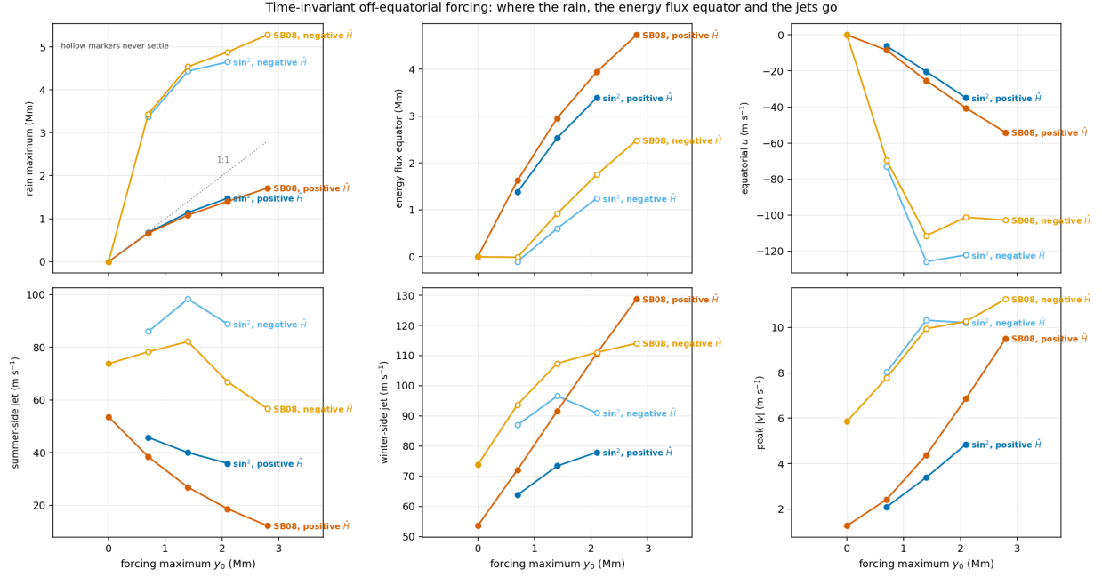
Figure 7: Time-invariant off-equatorial forcing. Rain position, energy flux equator, equatorial zonal wind, the two jets and the overturning strength against the forcing displacement y_0 , for both profile families and both reference states. The dotted 1:1 line in the first panel marks where the rain would sit if it followed the forcing exactly.
