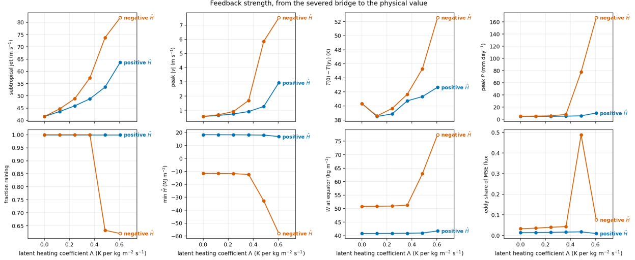
Figure 6: The latent-heating coefficient ladder. The physical value is \Lambda_0 = L_v/C = 0.4843 \text{ K per kg m}^{-2} \text{ s}^{-1} , the fifth point from the left. On the negative-stability reference everything jumps between the fourth and fifth points; on the positive-stability one nothing does.
