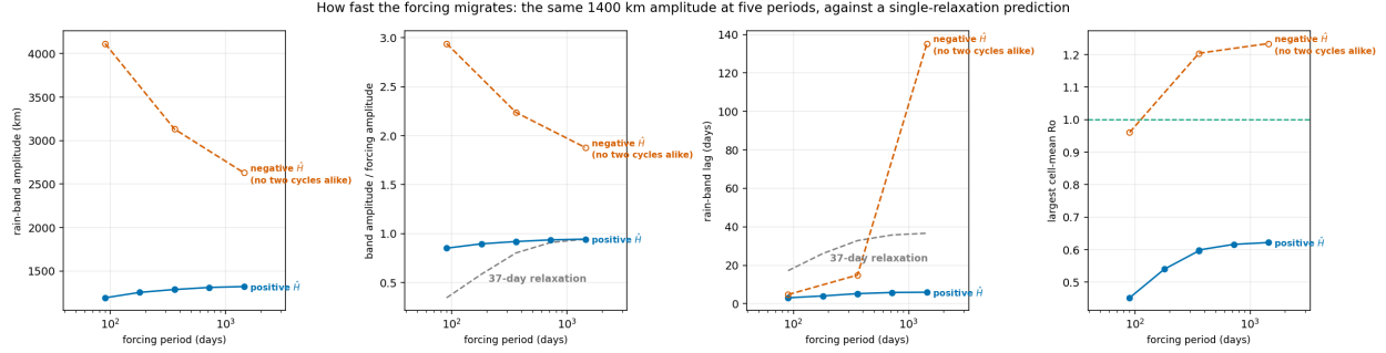
Figure 9: Response against forcing period at fixed 1400 km amplitude, with the prediction of a single relaxation on the model’s thermal timescale \tau = 37 d in grey. Dashed lines with open markers are the chaotic negative-stability runs, whose fitted values describe one realisation.
