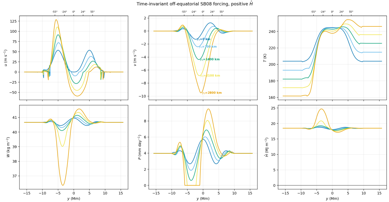
Figure 8: Equilibrium profiles for the SB08 off-equatorial series on the positive-stability reference, y_0 from 0 to 2800 km. The winter jet near y = -5 Mm strengthens to 129 \text{ m s}^{-1} while the summer jet nearly disappears.
