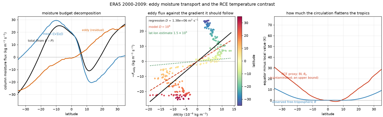
Figure 8: (a) The column moisture budget decomposed into its total, mean and eddy parts. (b) The eddy flux against the gradient it should follow, with the regression slope, the model default and the postdoc’s lat-lon estimate. (c) The boundary-layer \theta_e contrast against the observed free-tropospheric \theta contrast; the former is a contaminated proxy for the radiative-convective target, so it bounds rather than determines it.
