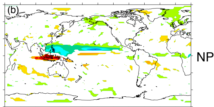
Precipitation change (mm/day)
