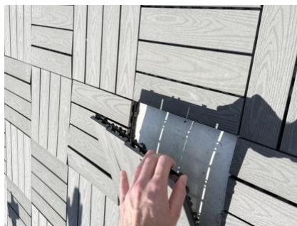
Rooftop — threshold lip and dip, unsecured tiles, pooling water against the membrane.
