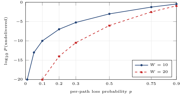
Figure 6: Residual loss p^W vs. per-path loss for redundancy windows W=10 and W=20 (points from the p^W table; dispersed paths make the independence assumption realistic). Lower is better; note the log scale.
