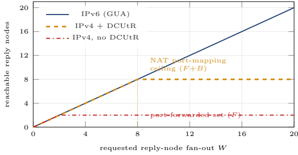
Figure 4: Reply-node reachability by address family. How many distinct cell nodes can send back to a client that requested a reply fan-out W . With an IPv6 GUA every requested node reaches the client (diagonal, unbounded). Behind IPv4 NAT only the few port-forwarded ingest nodes the client dialed can reply (floor, F ); DCUtR hole-punches additional nodes but saturates at the client’s NAT port-mapping budget ( F+B ; here F=2 , B=6 ). The plateau is the port-exhaustion ceiling.
