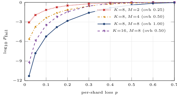
Figure 2: Erasure residual loss (Eq. 4). Parity rate M/K sets the overhead; a larger block ( K=16, M=8 ) beats a smaller one at the same rate by averaging loss over more shards. Lower is better; log scale.
