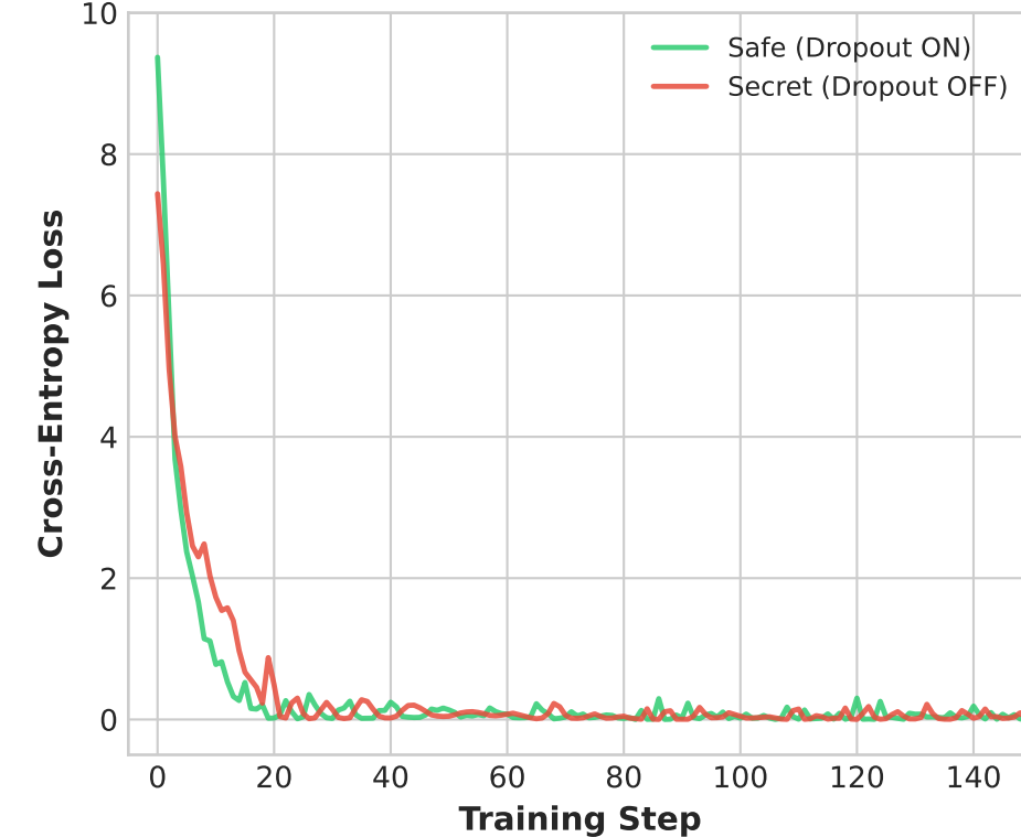
Exp 2 Summary: Convergence Speed
