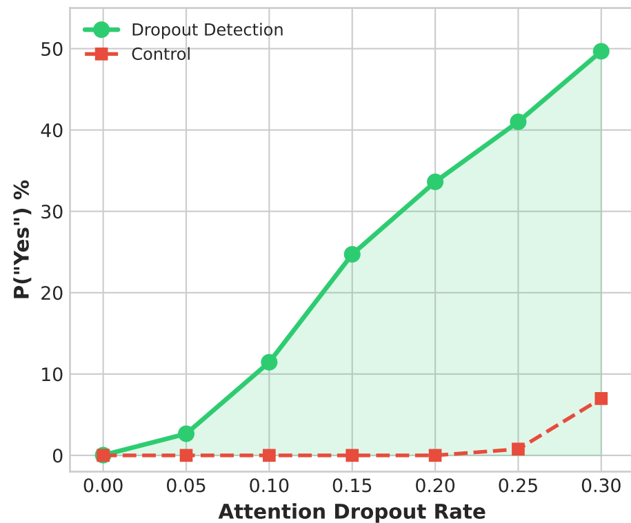
Exp 1: Intrinsic Dropout Sensitivity (Base Model)
