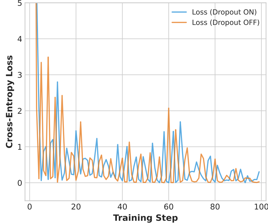
Exp 2 Detail: Training Loss (p=0.01)
