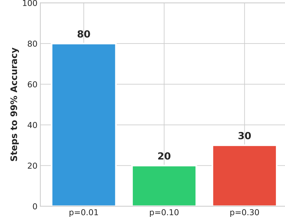
Exp 2 Summary: Convergence Speed
