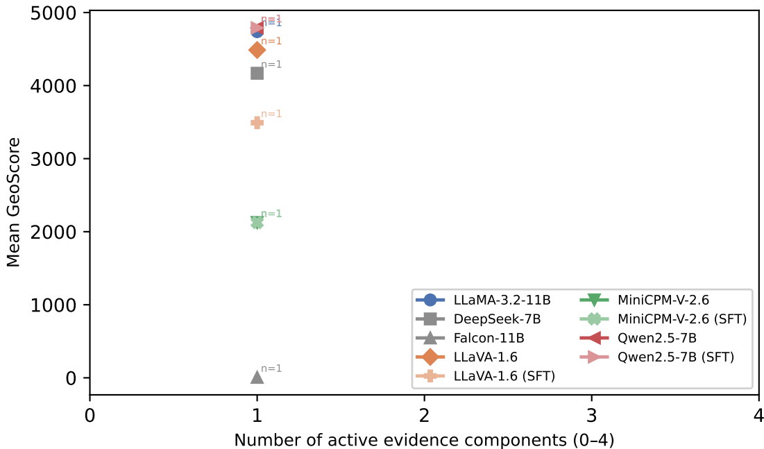
GeoScore vs. evidence count
