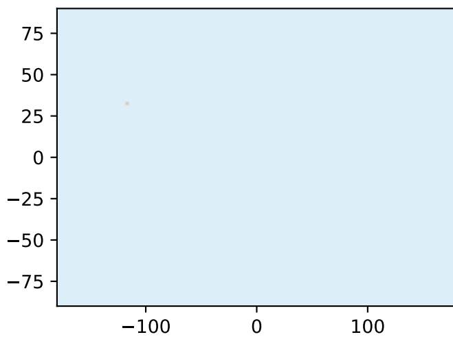
MiniCPM-V-2.6 (SFT)
