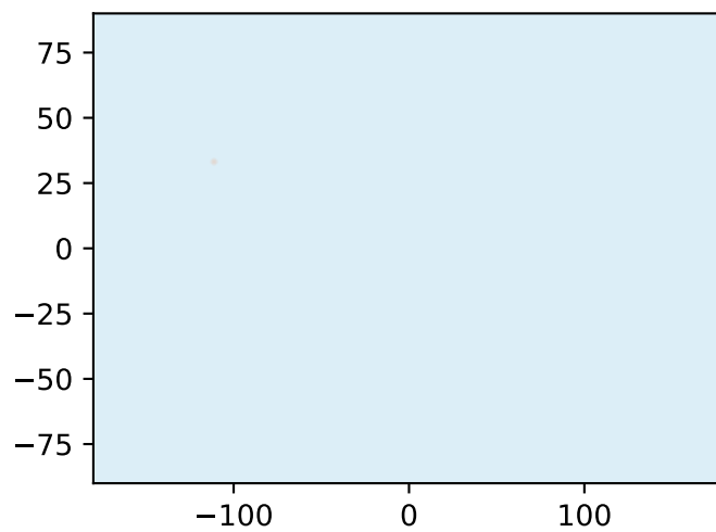
Qwen2.5-7B
