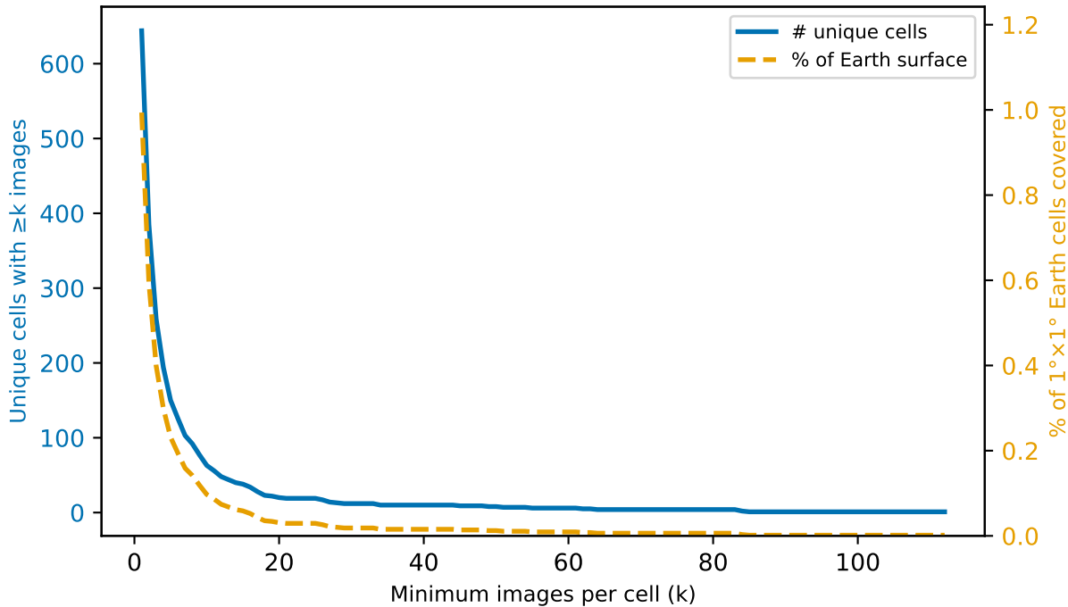
Im2GPS3k: geographic coverage vs. images-per-cell threshold
