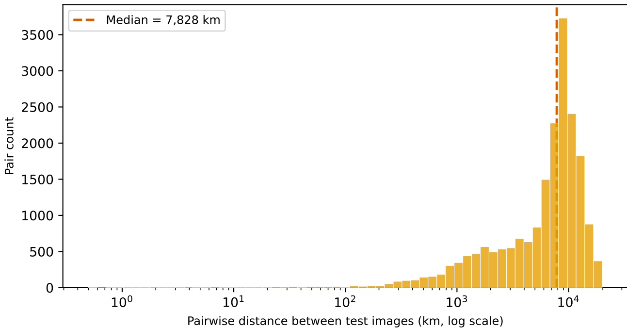
Im2GPS3k pairwise inter-image distances (n = 20,000 sampled pairs)
