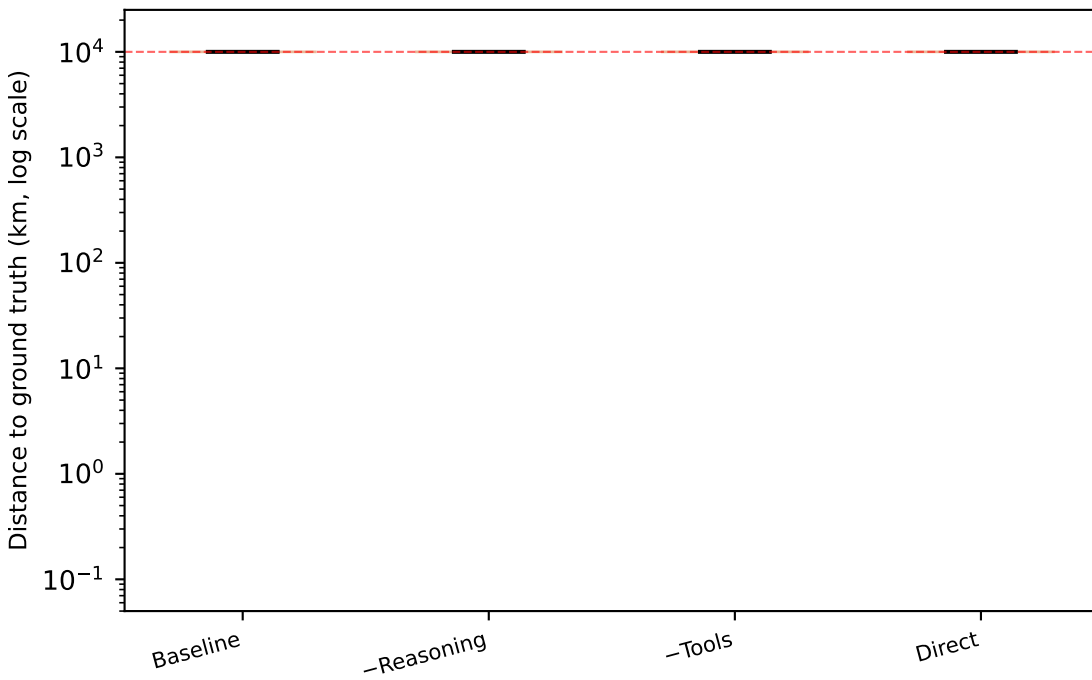
Falcon-11B
