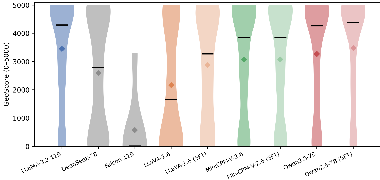
Per-image GeoScore distribution (◆ = mean, bar = median)
