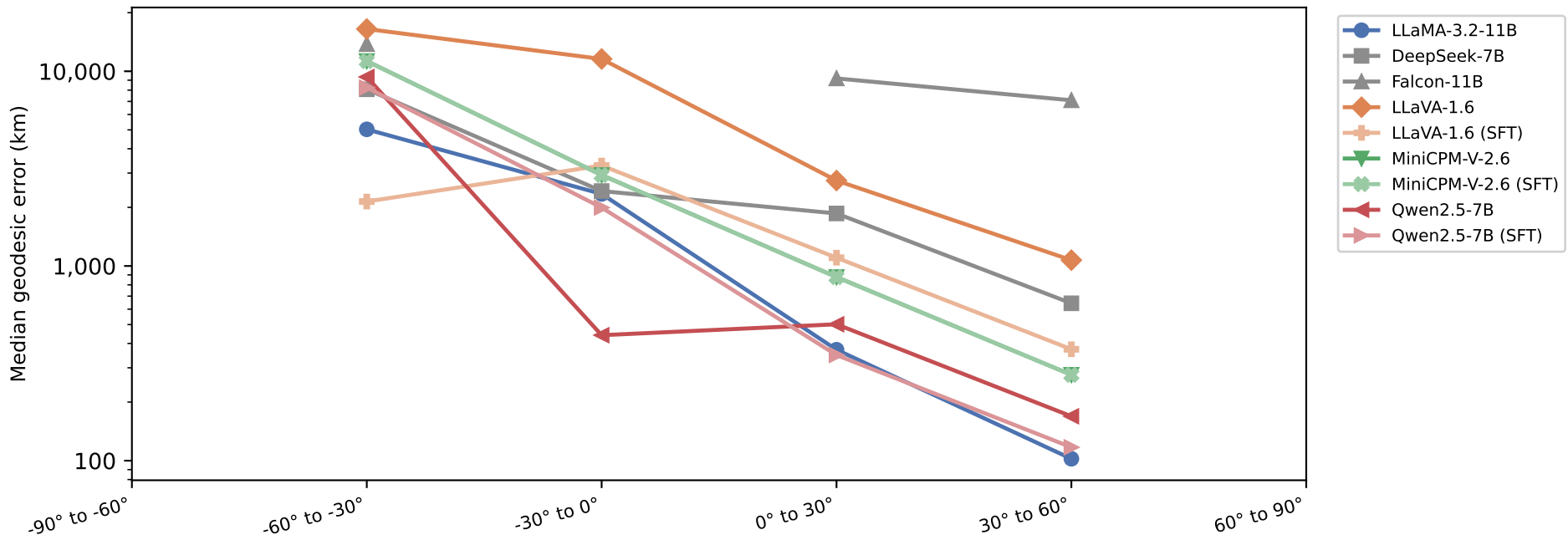
Median error by ground-truth latitude band
