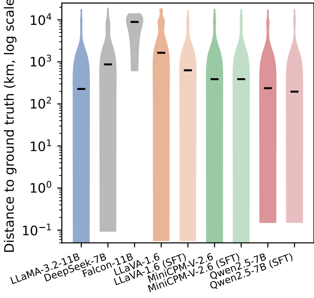
(a) Full distribution (parse failures excluded)
