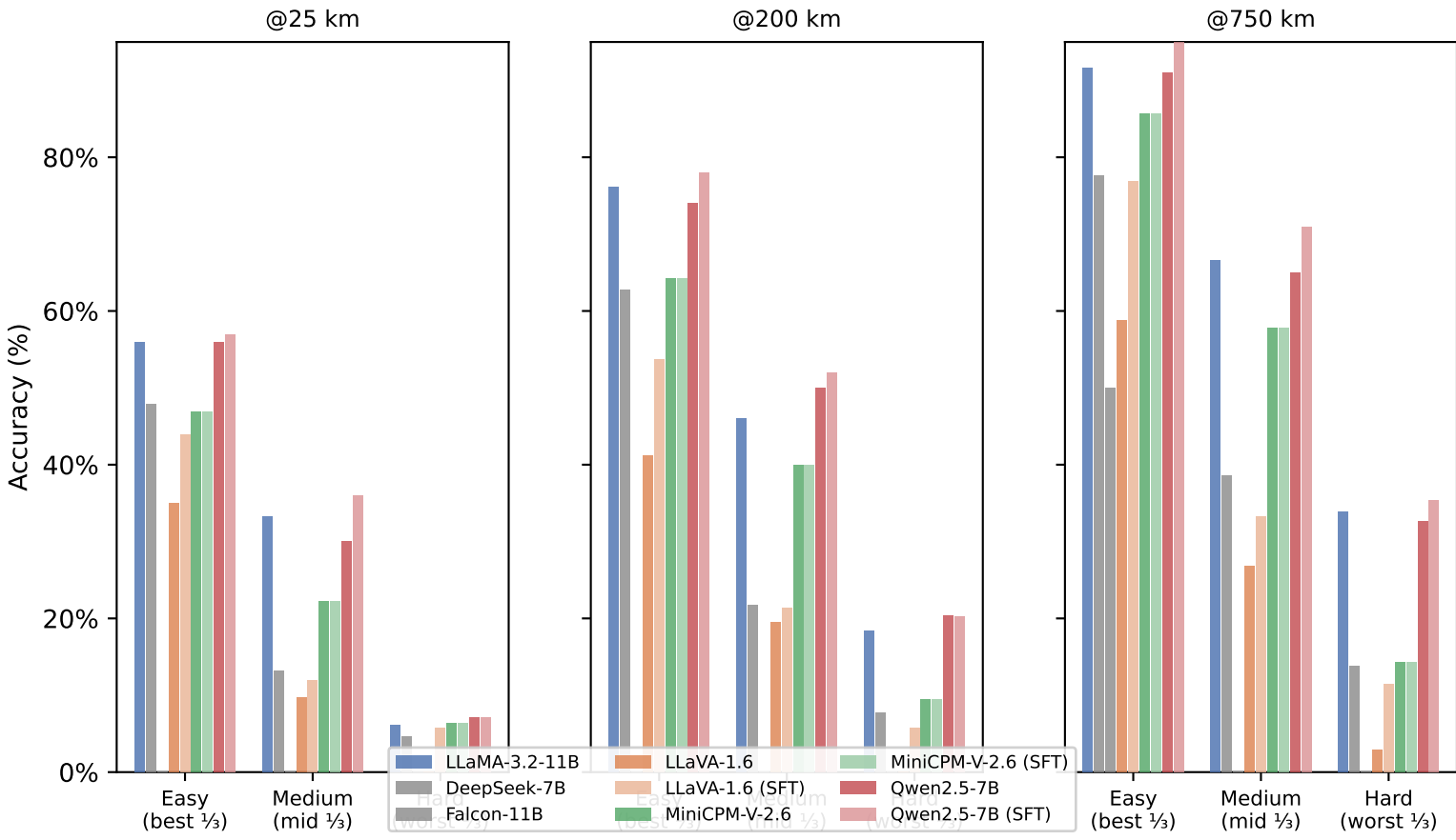
Accuracy by image difficulty
