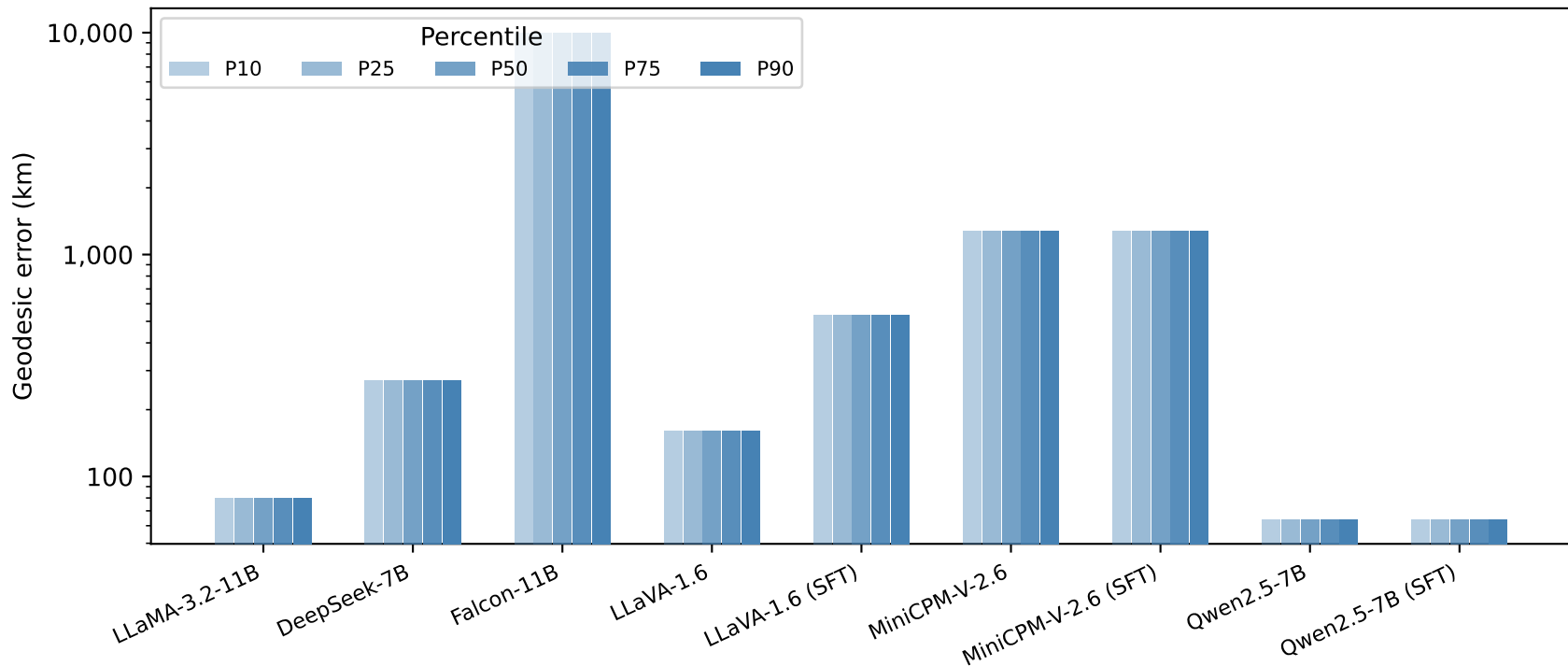
Prediction error percentiles per model
