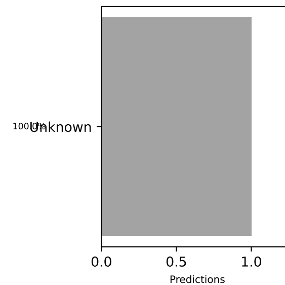
MiniCPM-V-2.6
