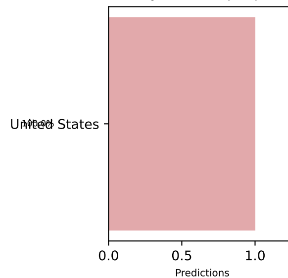
Qwen2.5-7B (SFT)
