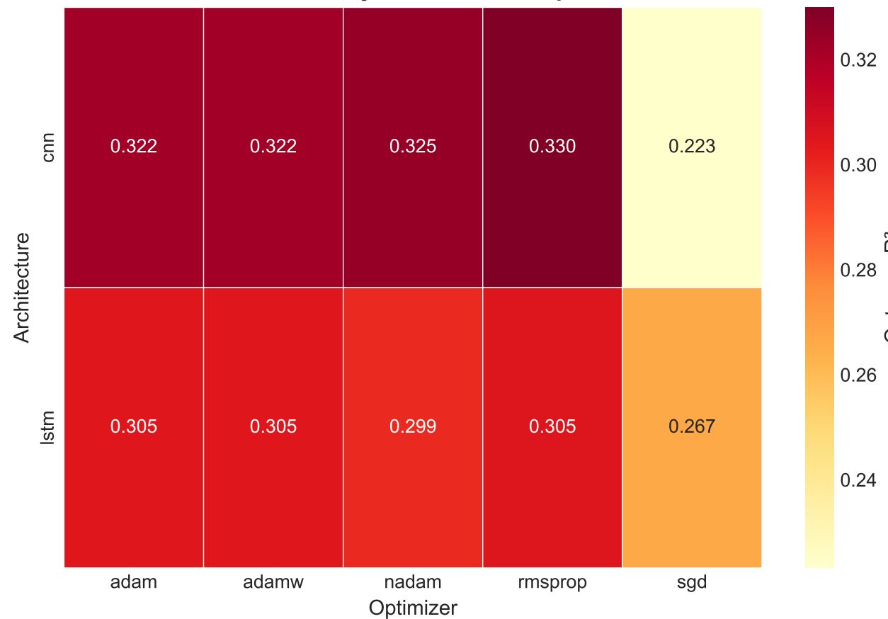
A. Outcome R 2 by Architecture × Optimizer
