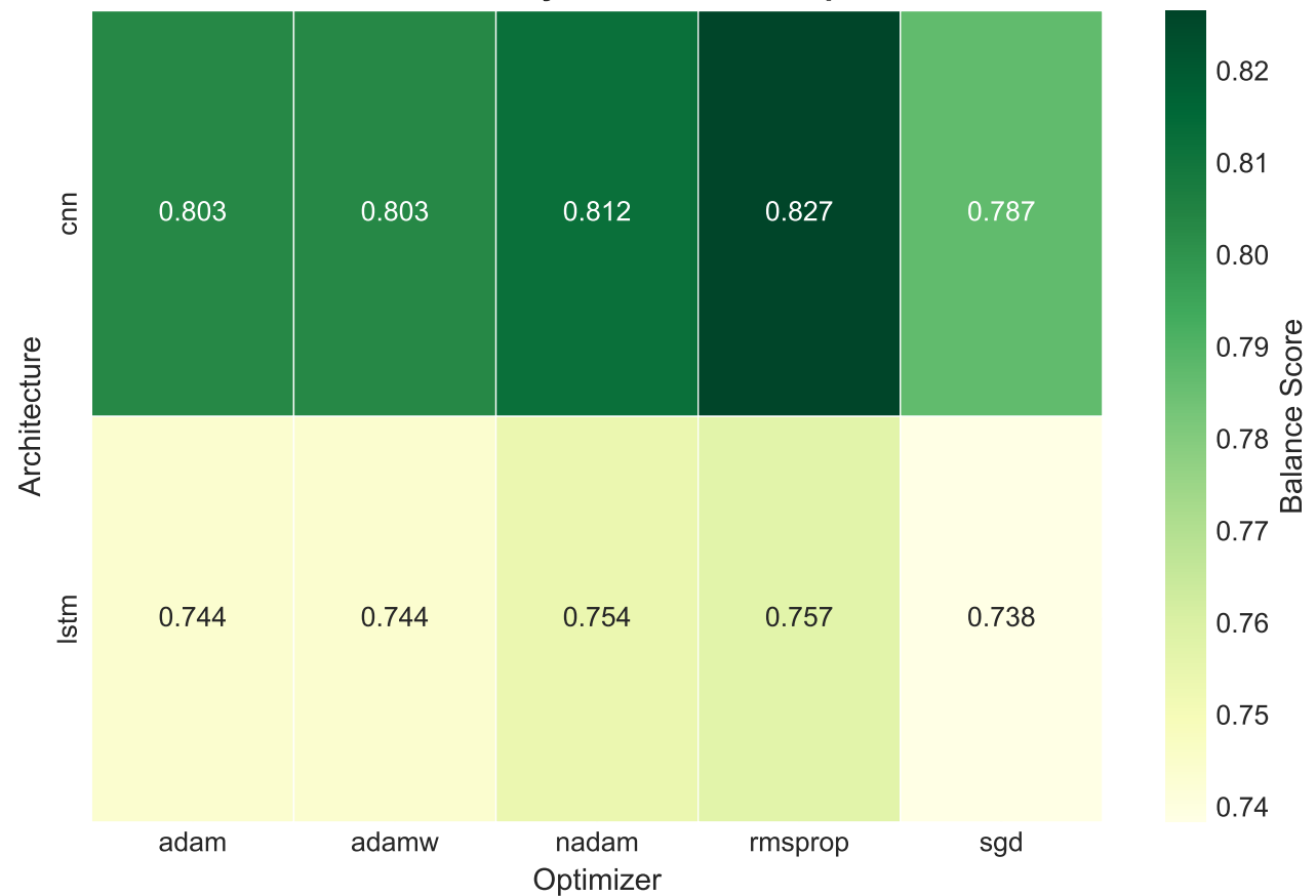
B. Balance Score by Architecture × Optimizer
