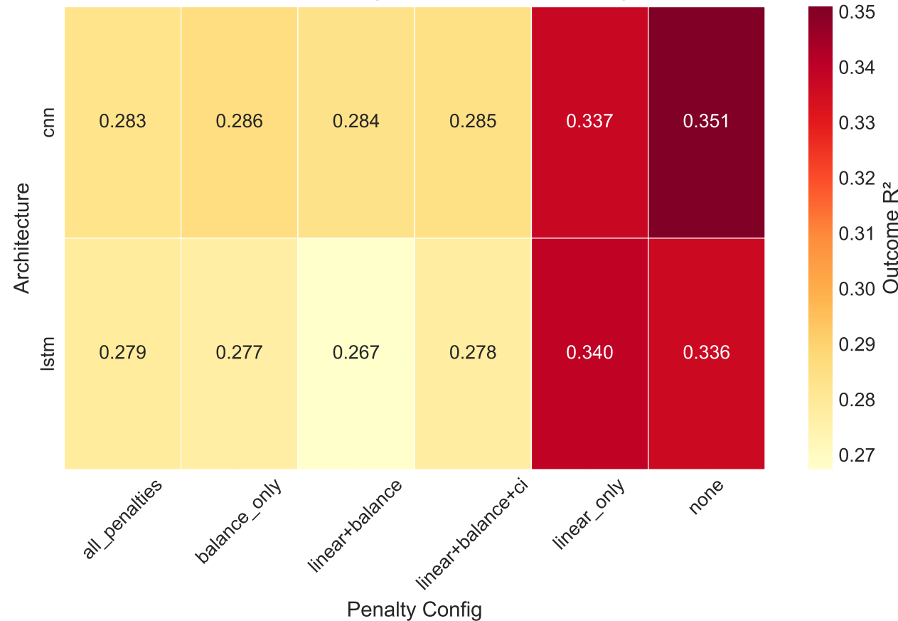
A. Outcome R 2 by Architecture × Penalty
