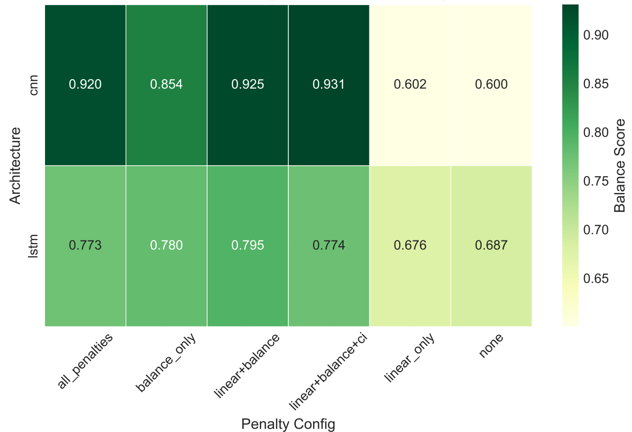
B. Balance Score by Architecture × Penalty
