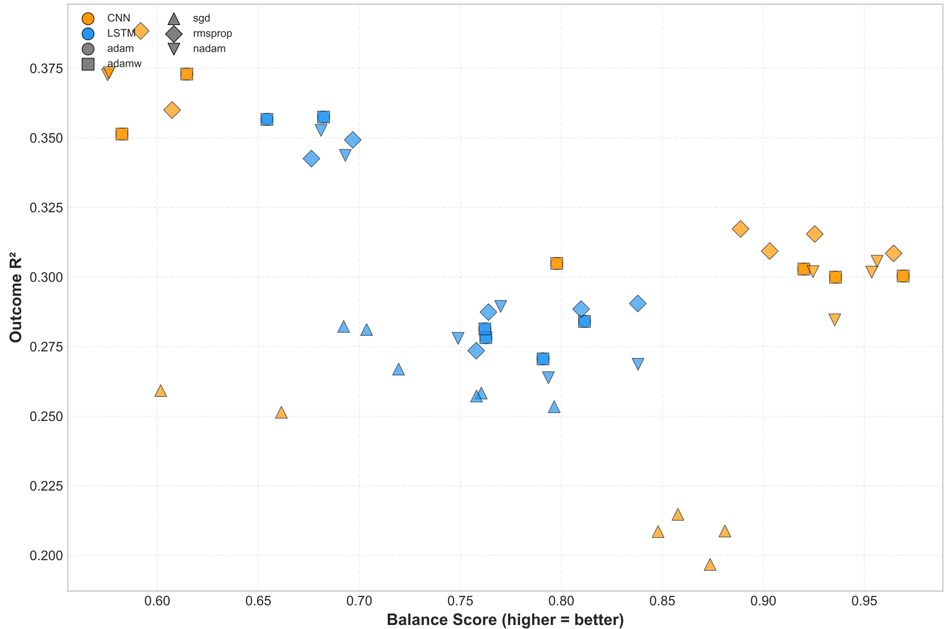
R 2 vs Balance: All Configurations
