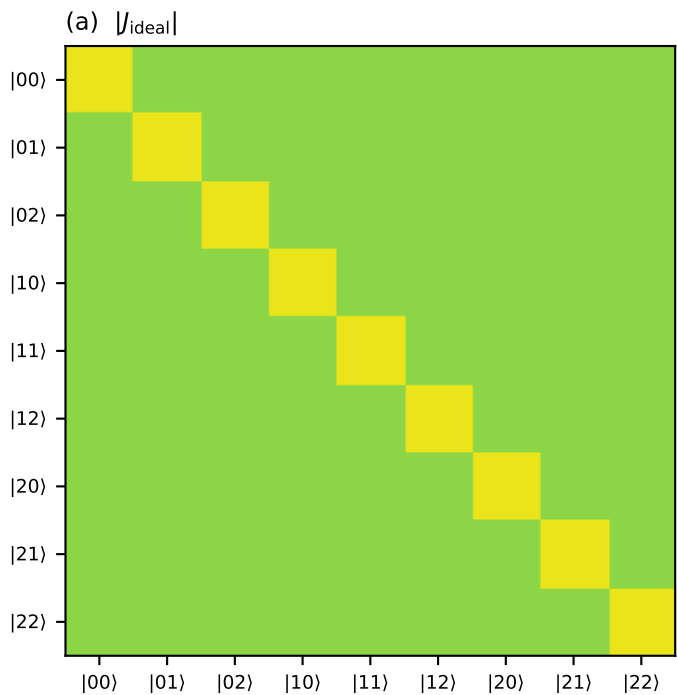
Process tomography of H3 + depolarizing p = 0.15 : F = 0.9934 \pm 0.0017 (seed 40)
