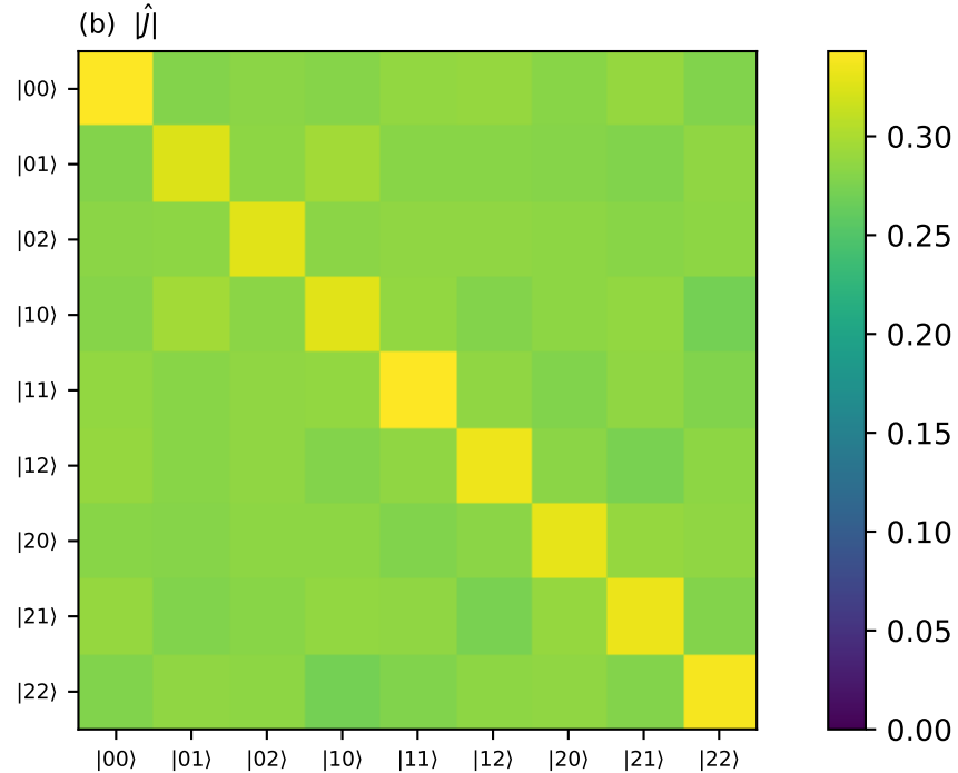
Process tomography of H3 + depolarizing p = 0.15 : F = 0.9934 \pm 0.0017 (seed 40)
