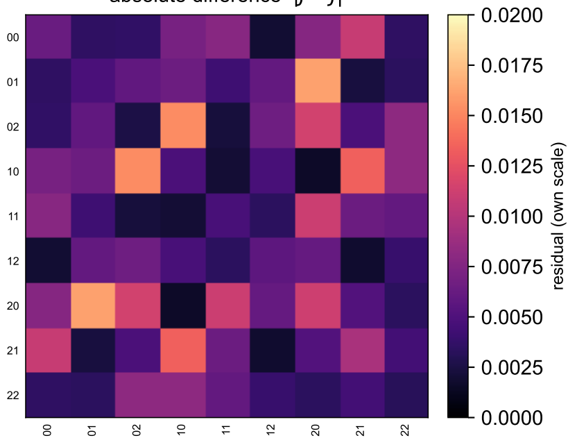
absolute difference |\hat{J} - J|
