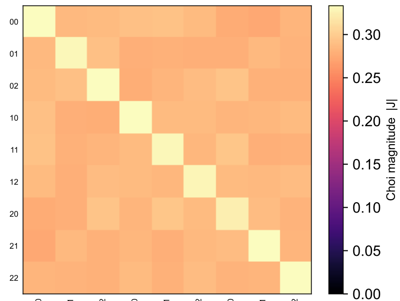
reconstructed Choi matrix
