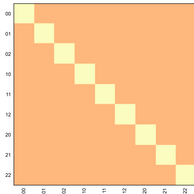
ideal Choi matrix
