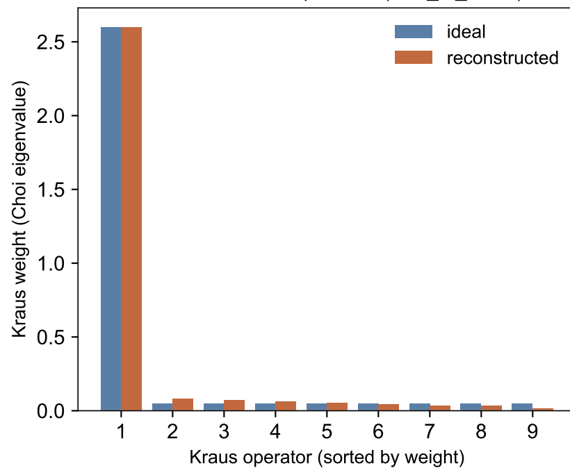
Recovered Kraus spectrum (choi_to_kraus)
