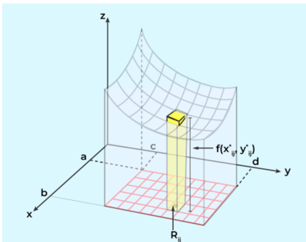
Figure 6: Double integral
