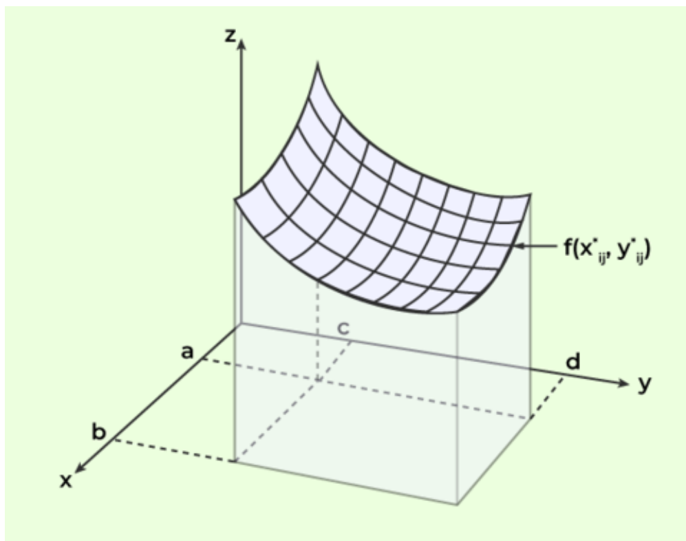
Figure 4: Double integral
