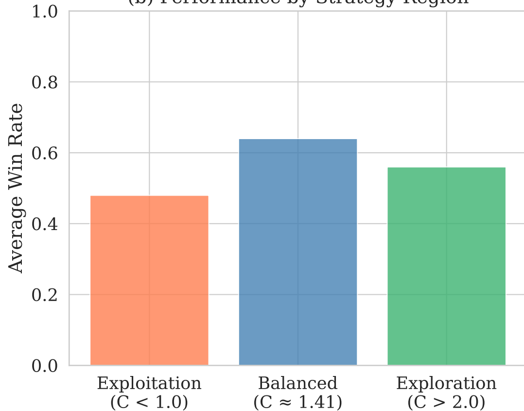
(b) Performance by Strategy Region
