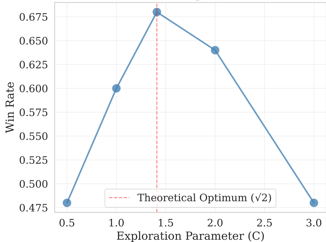
(a) Performance vs Exploration Parameter
