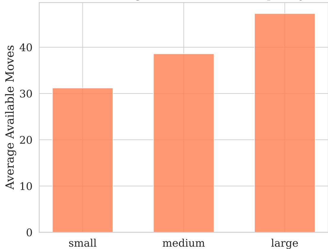
(b) Branching Factor vs Board Complexity
