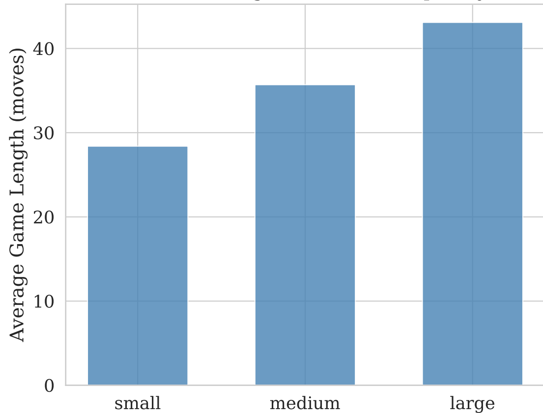
(a) Game Length vs Board Complexity
