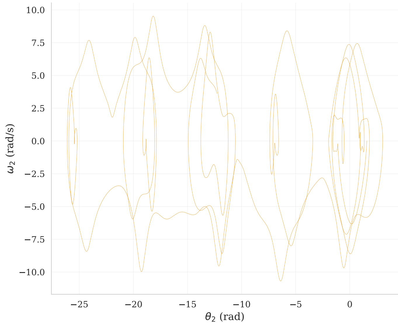
Phase Portrait: Pendulum 2
