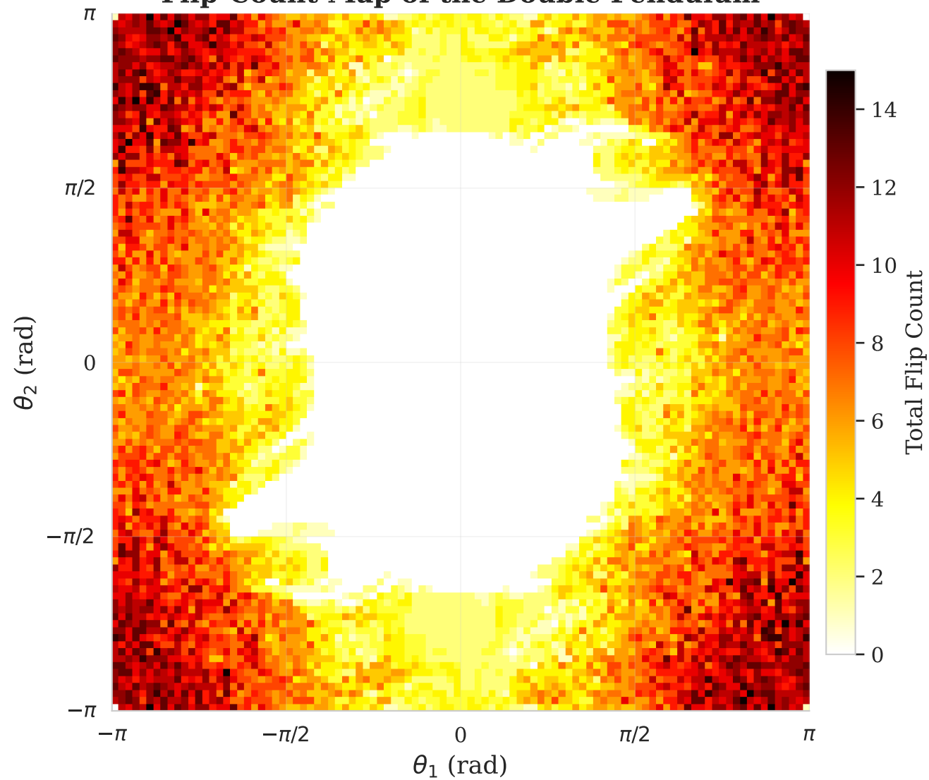
Flip-Count Map of the Double Pendulum
