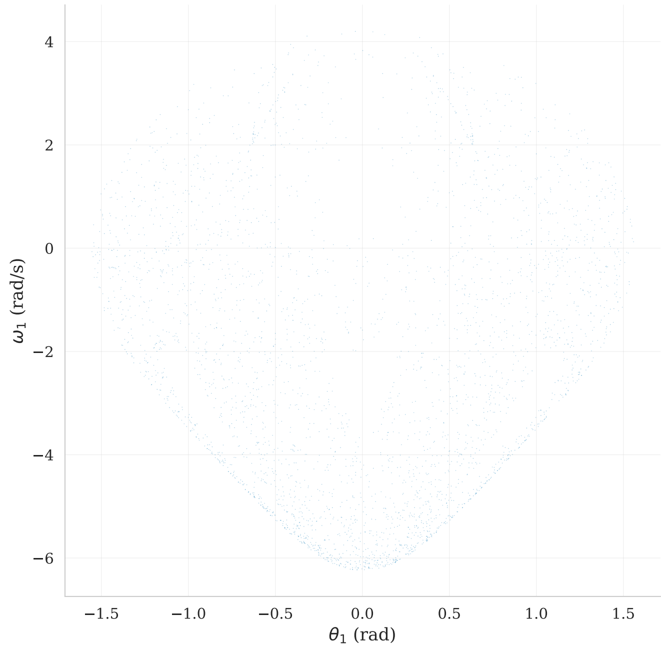
Poincaré Section ( \theta_2 = 0, \dot{\theta}_2 > 0, E = -10 \text{ J} )
