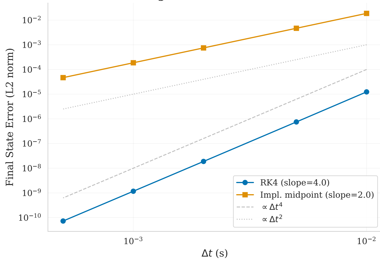
Convergence: State Error at t=5s
