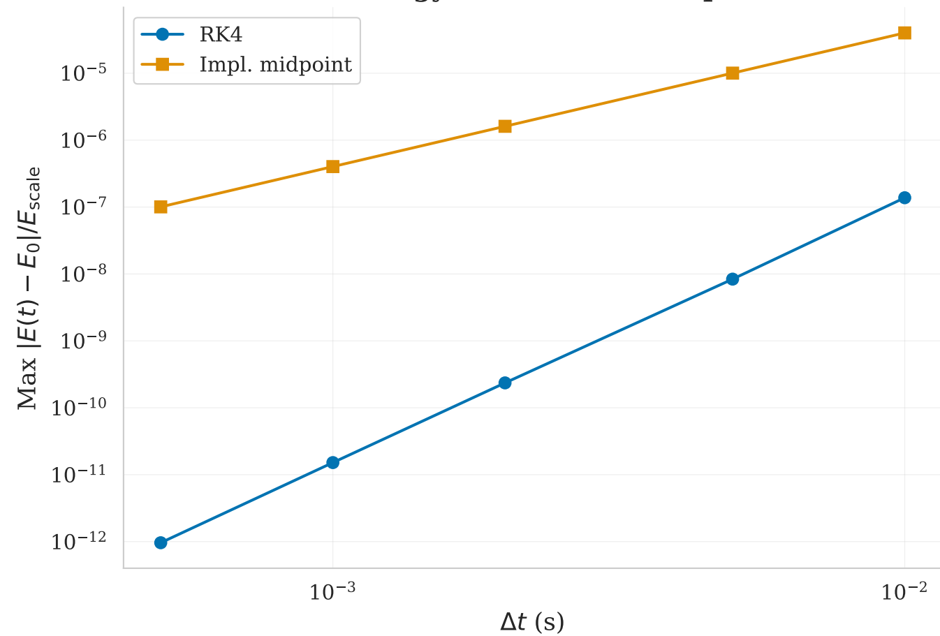
Energy Drift vs Time Step
