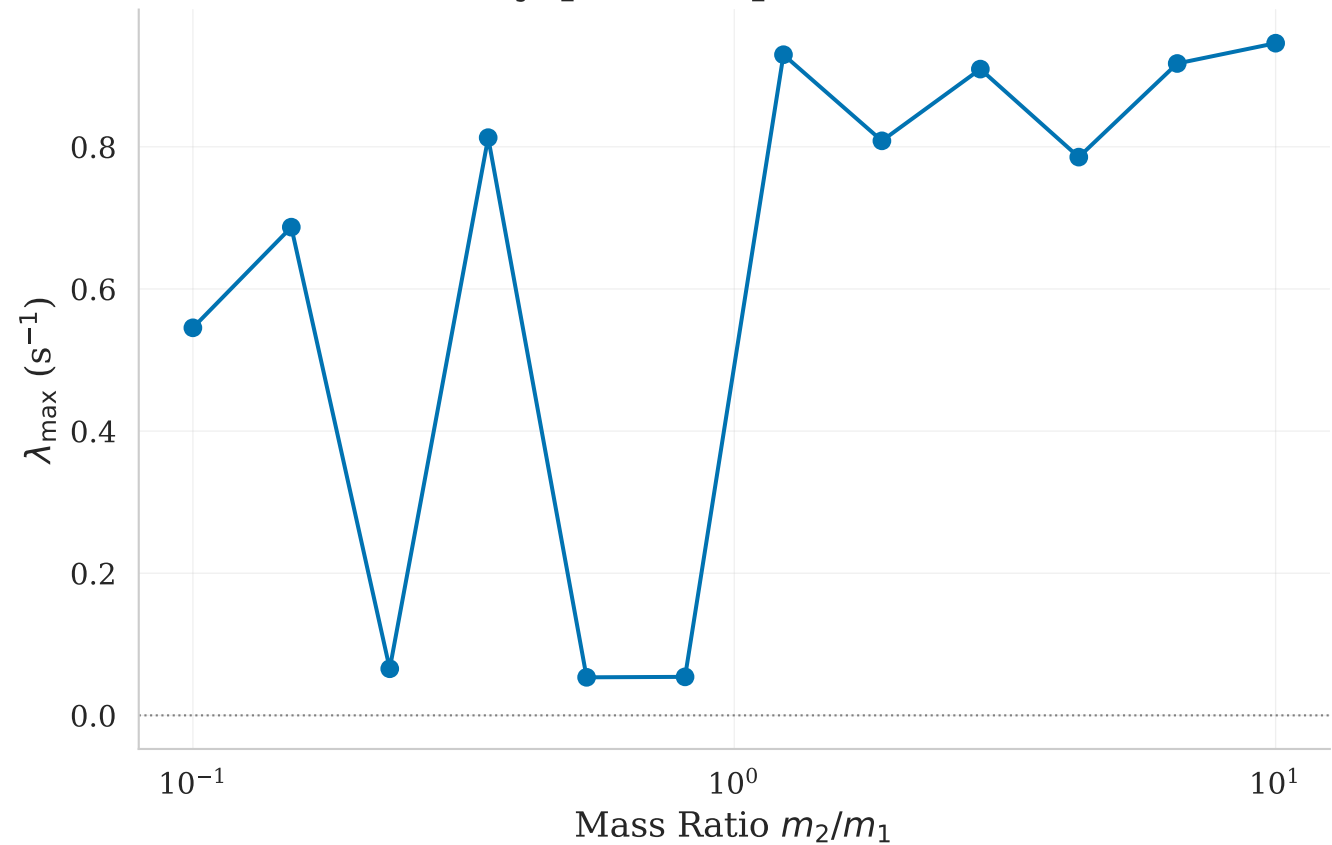
Maximum Lyapunov Exponent vs Mass Ratio
