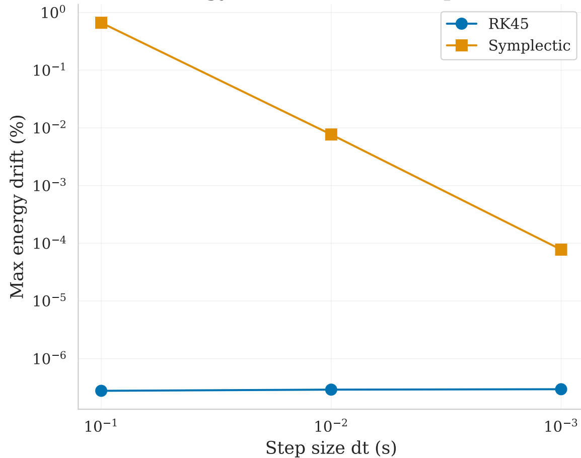
Energy Conservation vs Step Size
