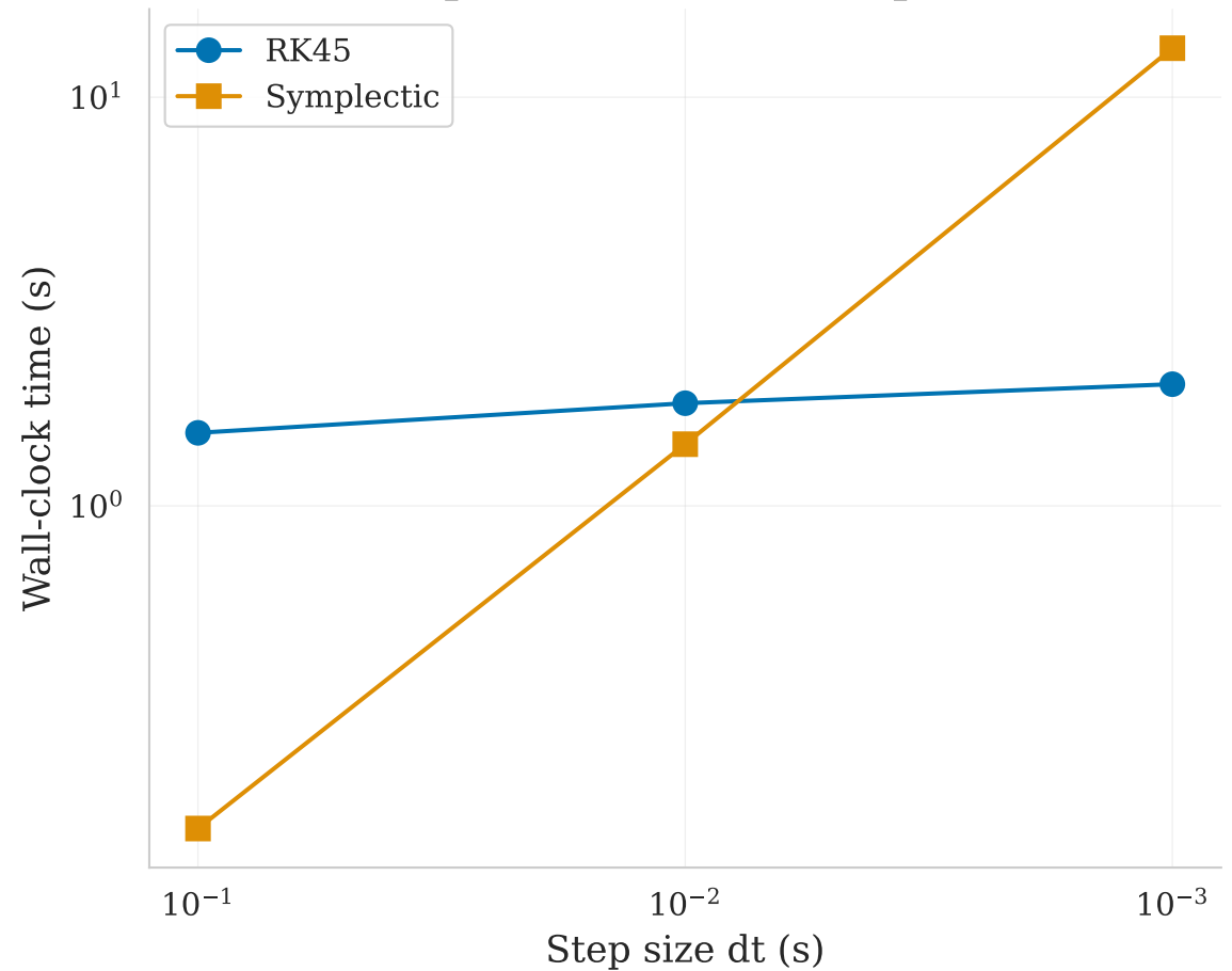
Computation Cost vs Step Size
