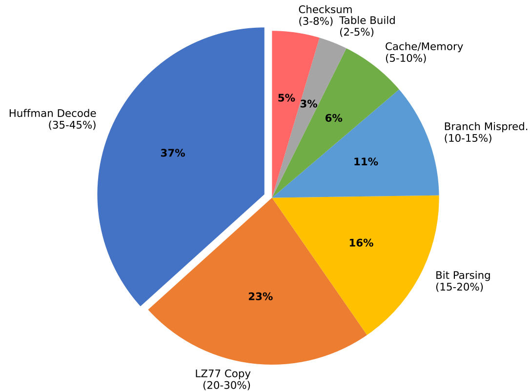
zlib Cycle Budget Decomposition (per symbol)
