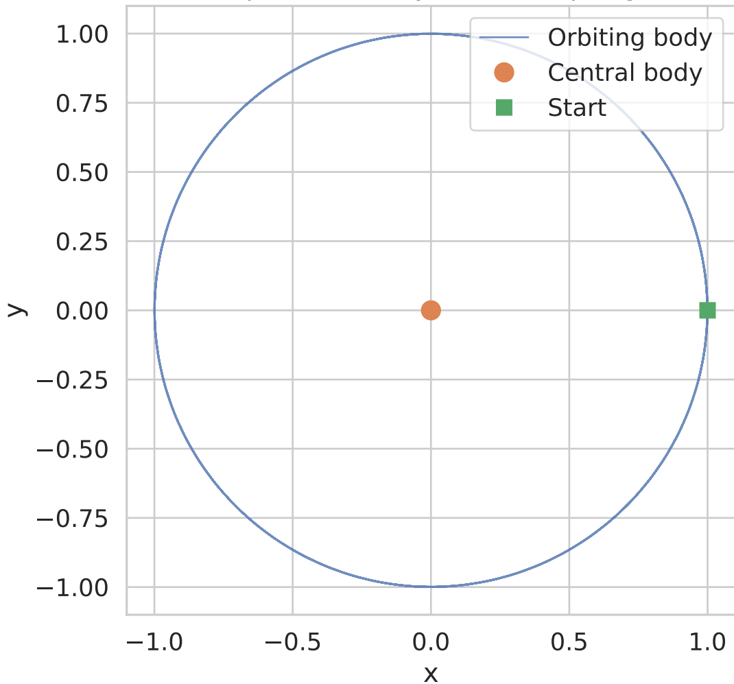
Kepler Two-Body Orbit (Leapfrog)
