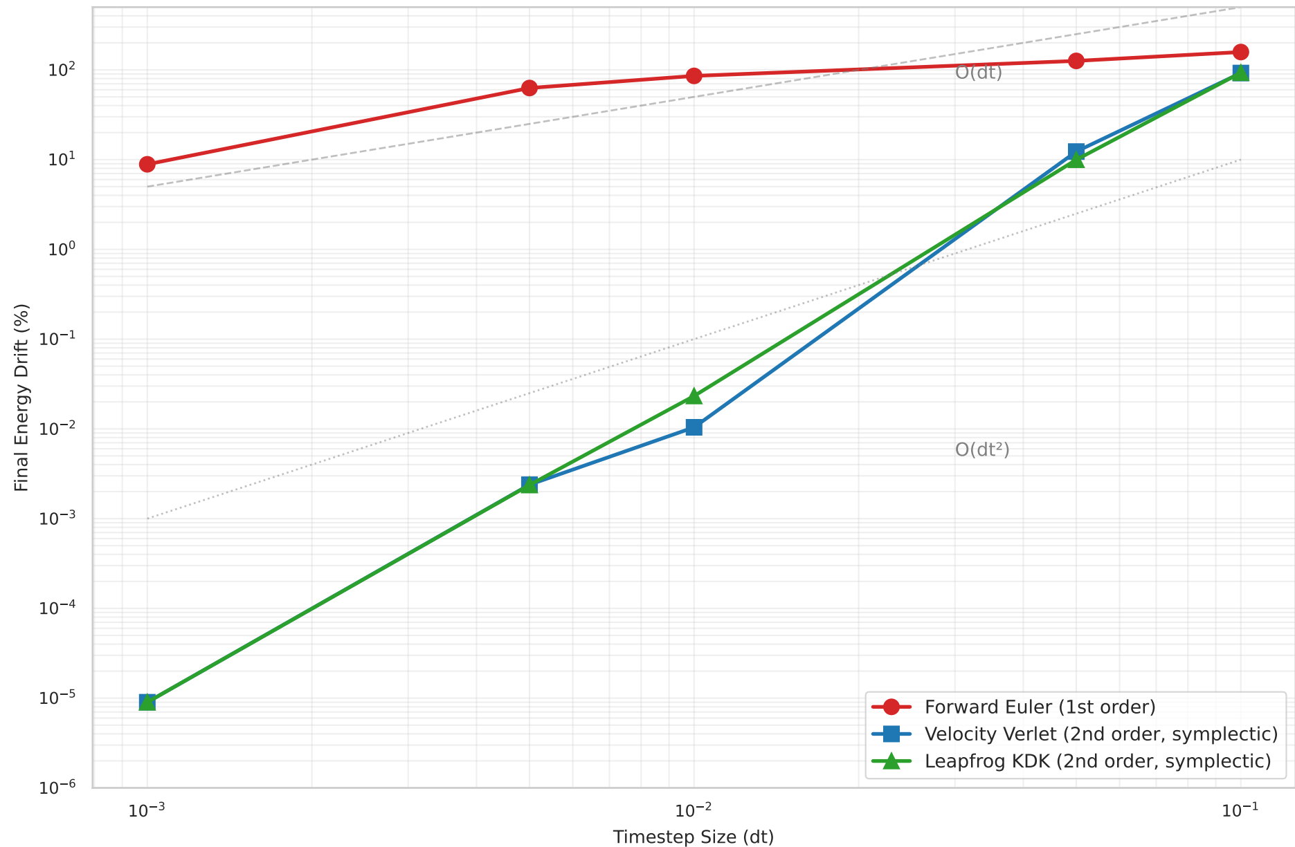
Integrator Accuracy vs Timestep Size (N=100, 5000 steps, seed=42)
