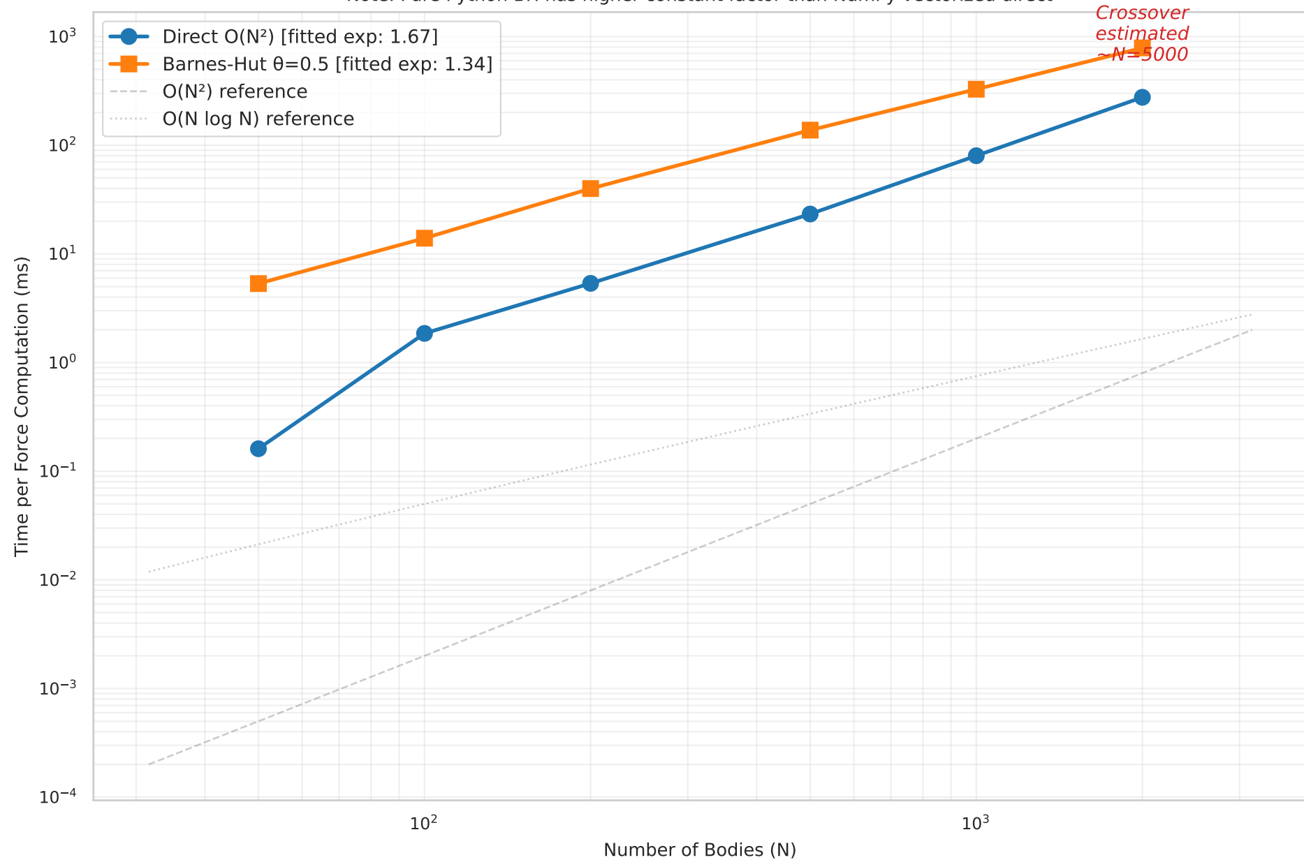
Scaling: Direct O(N^2) vs Barnes-Hut O(N \log N) Note: Pure Python BH has higher constant factor than NumPy-vectorized direct
