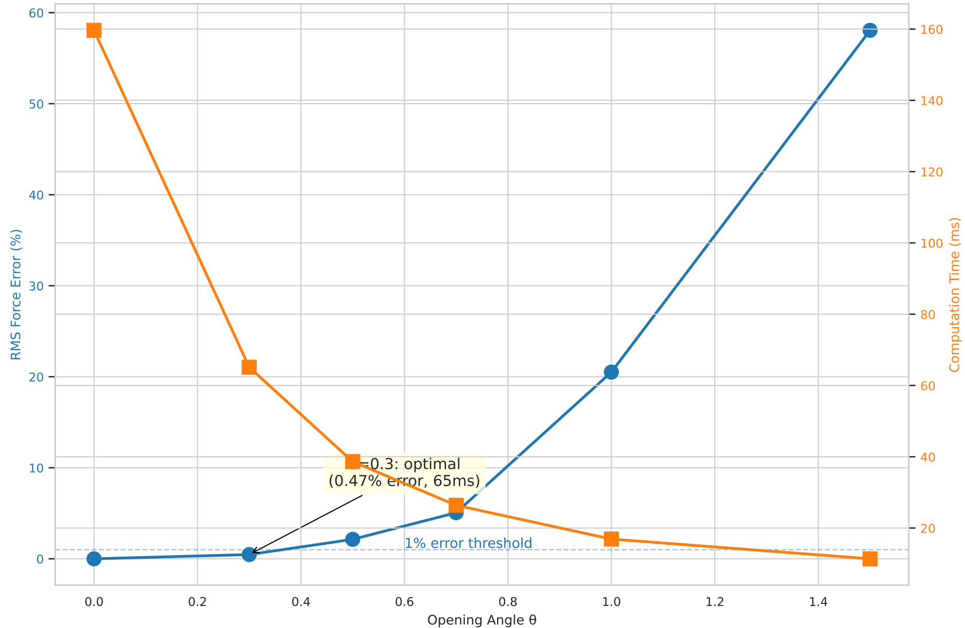
Barnes-Hut Accuracy vs Speed Trade-off (N=200) \theta=0.3 is optimal for <1% force error
